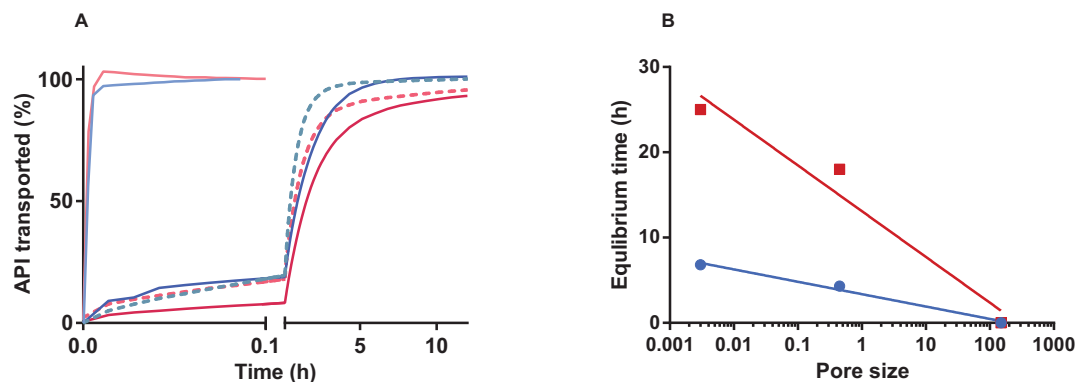
Fig. 2. (A) Transport of metoprolol and diclofenac in aqueous solution across three diffusion barriers. Metoprolol across the nylon mesh filter, 150 μm pores, (—); the polyvinylidene fluoride filter, 0.45 μm pores, (---); and the cellulose-based dialysis membrane, approximate pore size 0.003 μm, (—). Diclofenac across the nylon mesh filter (—); the polyvinylidene fluoride filter (---), and the cellulose-based dialysis membrane (—). All experiments were carried out at 37 °C with a stirring rate of 400 rpm. (B) Correlation between equilibrium time (h) and pore size described with a nonlinear semi-log function for diclofenac and metoprolol, y = 3.4 - 1.5 \cdot \log x , R^2 = 0.98 , and y = 13 - 5.4 \cdot \log x , R^2 = 0.96 , respectively. Metoprolol observed values (■) and the non-linear semi-log function values (—); diclofenac observed values (●) and the non-linear semi-log function values (—).
