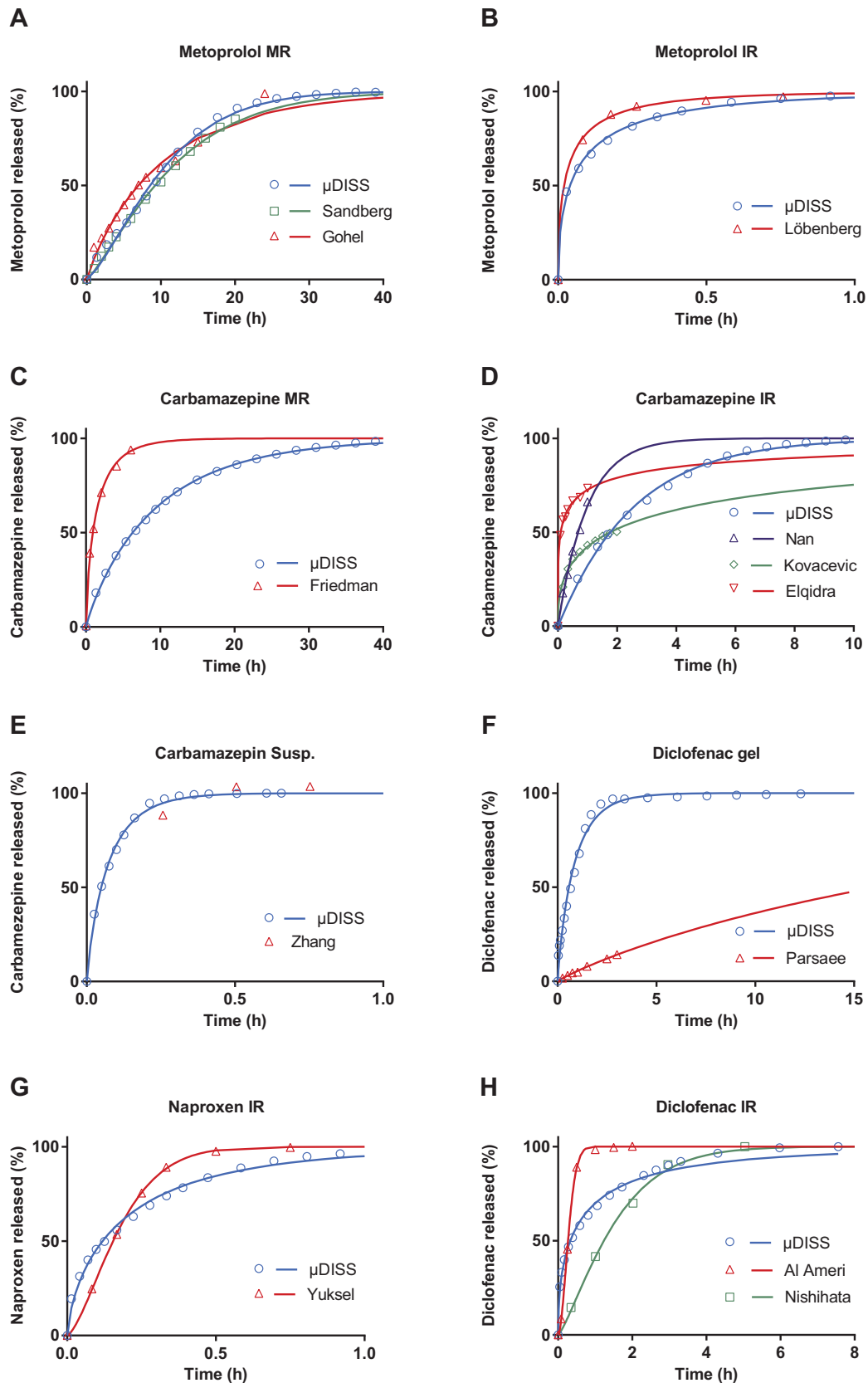
Fig. 4. In vitro drug release using data acquired with the novel, miniaturized, \mu DISS TM in vitro release method and historical in vitro data. Symbols represent the observed data and lines represent WinNonlin curve fitting of the Weibull function. (A) Release profile for metoprolol from a slurry of modified-release (MR) pellets using data from the miniaturized method and historical data (Gohel et al., 2009; Sandberg et al., 1988). (B) Release profile for metoprolol from a slurry of immediate-release (IR) metoprolol using miniaturized-method data and historical data (Löbenberg et al., 2005). (C) Release profile for carbamazepine from a slurry of MR carbamazepine using miniaturized-method data and historical data (Friedman et al., 2000). (D) Release profile for carbamazepine from a slurry of IR carbamazepine using miniaturized-method data and historical data (Elqidra et al., 2004; Kovacevic et al., 2008; Nan et al., 2012). (E) Release profile for carbamazepine from a carbamazepine oral suspension using miniaturized-method data and
