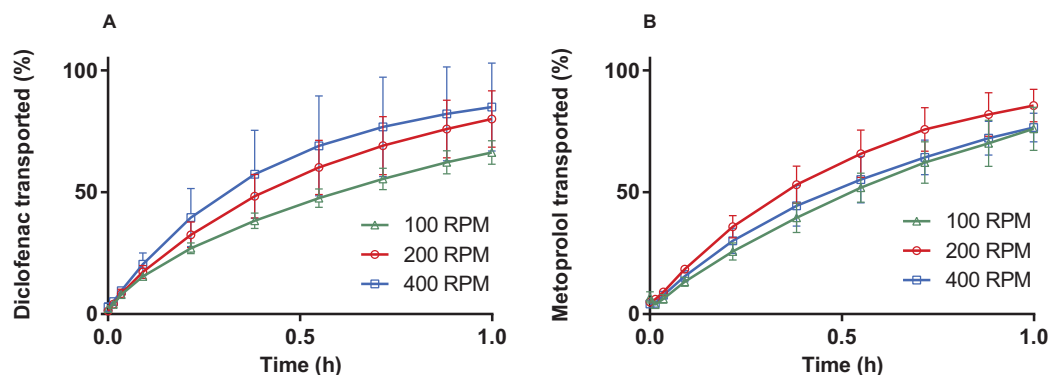
Fig. 3. (A) Effect of stirring rate on the transport of diclofenac in aqueous solution across the diffusion barrier. (B) Effect of stirring rate on the transport of metoprolol in aqueous solution across the diffusion barrier. Both experiments were performed at 37 °C with a polyvinylidene fluoride filter (0.45 μm pores) as diffusion barrier.
