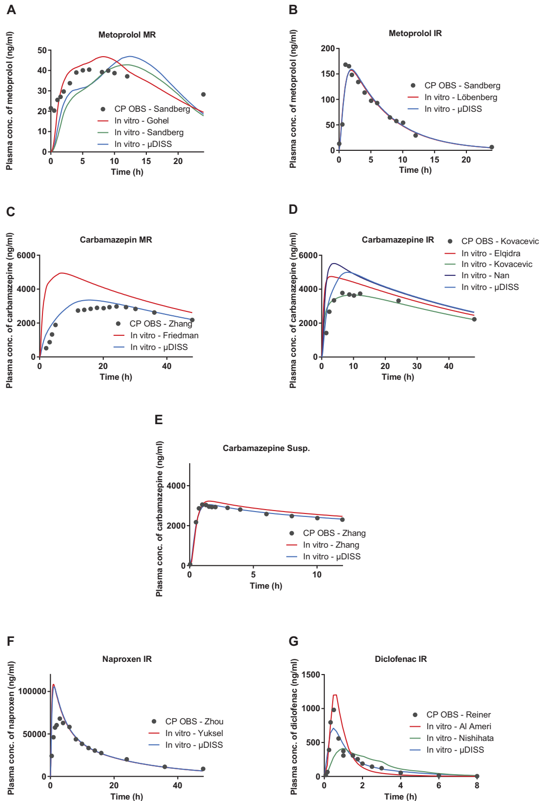
Fig. 5. Historical in vivo drug concentrations in plasma over time (CP OBS) and simulated (GI-Sim) in vivo plasma concentration-time profiles based on in vitro data obtained from the miniaturized method ( \mu DISS TM ) (data acquired with a nylon mesh, pore size 150 \mu m) and historical sources. Symbols represent historical CP OBS, lines represent simulated plasma concentrations. (A) observed data from Sandberg et al. (1988), simulated red line data from Gohel et al. (2009), simulated green line data from Sandberg et al. (1988), and simulated blue line data from the miniaturized method. (B) observed data from Sandberg et al. (1988), red line data from Löbenberg et al. (2005) and blue line data from the miniaturized method. (C) observed data from Zhang et al. (2011), red line data from Friedman et al. (2000), and blue line data from the miniaturized method. (D)
