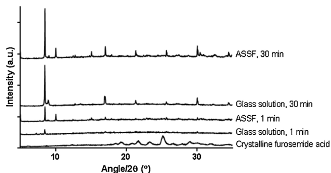
Fig. 4. XRPD of amorphous sodium salt of furosemide (ASSF) in glass solution at 1 and 30 min as found in Fig. 2 and the XRPD diffractograms for pure ASSF after 1 and 30 min of dissolution in a simulated intestinal medium at pH 6.5 (Nielsen et al., 2013b). As reference the diffractogram of crystalline furosemide acid has been added.
