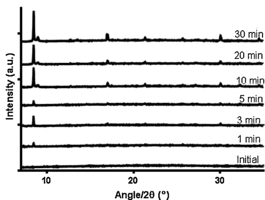
Fig. 3. XRPD of amorphous sodium salt of furosemide (ASSF) in glass solution following 1, 3, 5, 10, 20, and 30 min of dissolution on a \mu DISS profiler in a simulated intestinal medium pH 6.5. Diffractogram of ASSF in the glass solution before dissolution is shown for reference.
