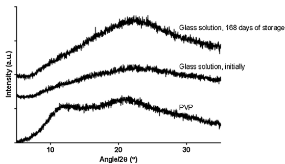
Fig. 2. XRPD diffractograms of the glass solution of amorphous sodium salt of furosemide (ASSF) and PVP initially after spray drying and after 168 days of storage at 20 °C and 0% RH. As reference the diffractogram of PVP is also shown.
